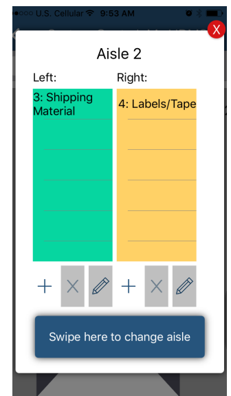
Item Locator Screen
